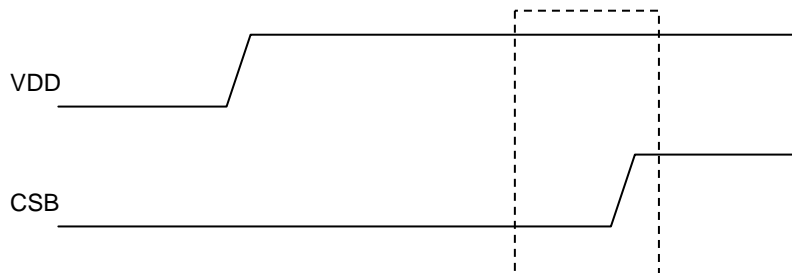
Figure 23. CSB timing
