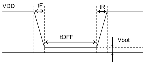
Figure 22. Power ON/OFF waveform
