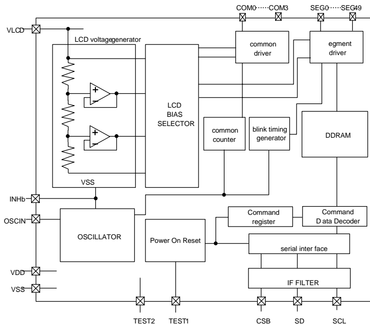
Figure 2. Block Diagram
