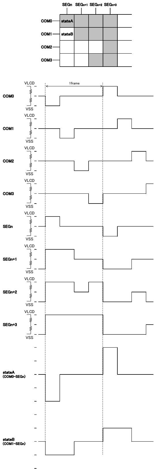
Figure 15.LCD waveform in line inversion (1/2bias) Figure 16. LCD waveform in frame inversion (1/2bias)
