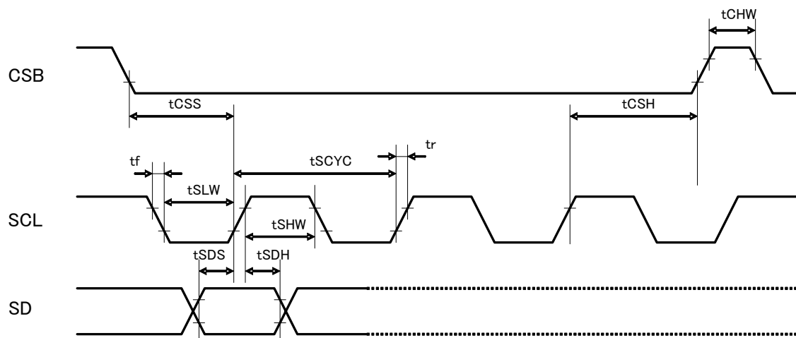
Figure 4. Interface Timing
