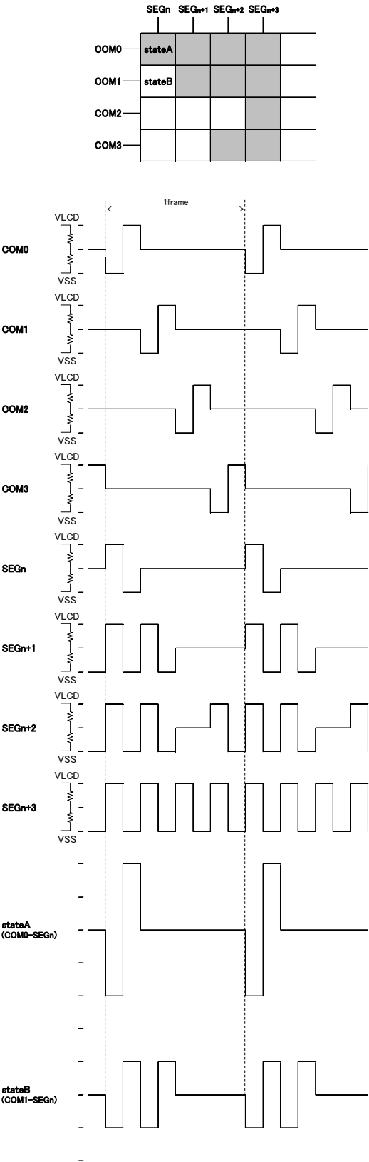
Figure 15.LCD waveform in line inversion (1/2bias) Figure 16. LCD waveform in frame inversion (1/2bias)
